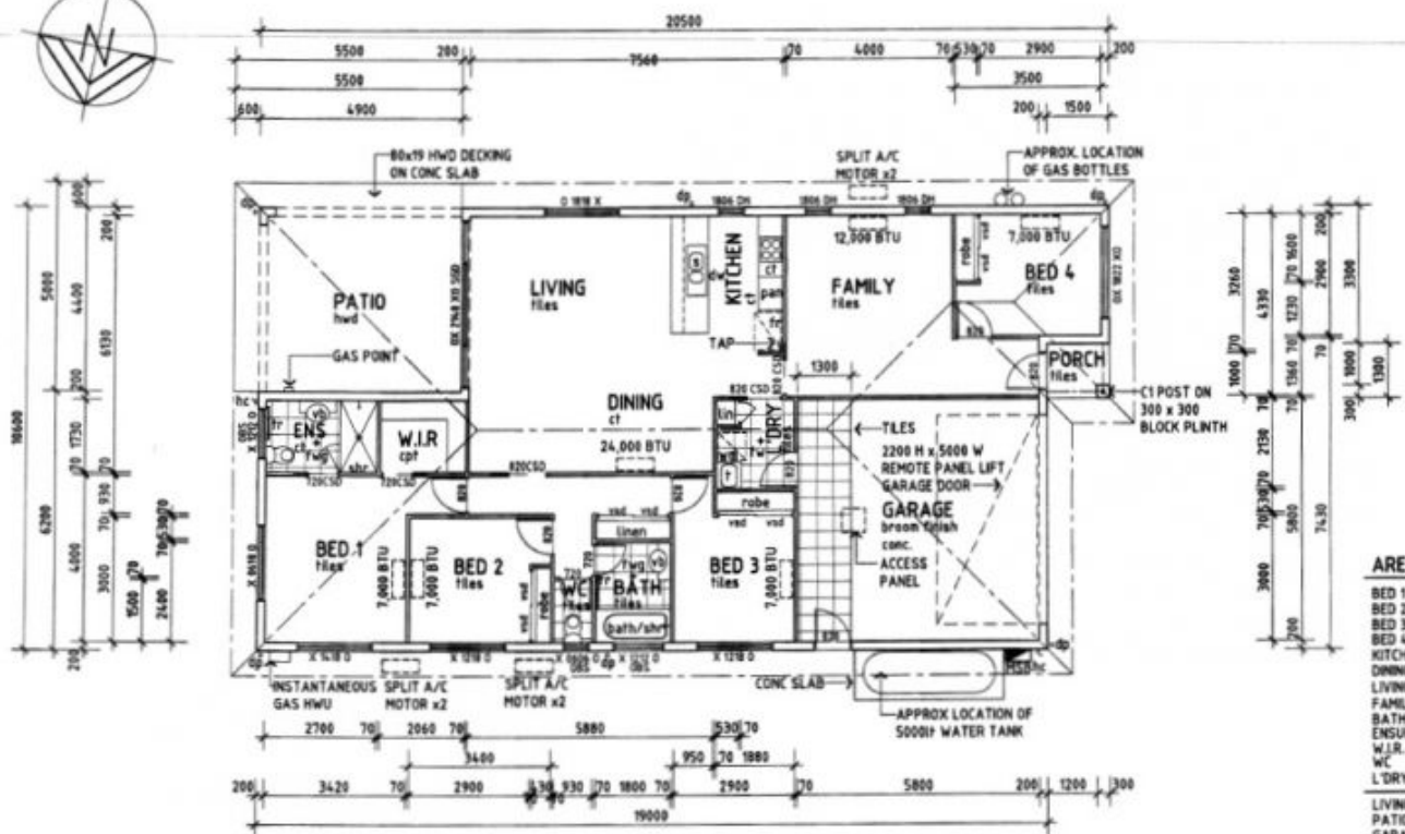
1 FLOOR PLAN 1:100
