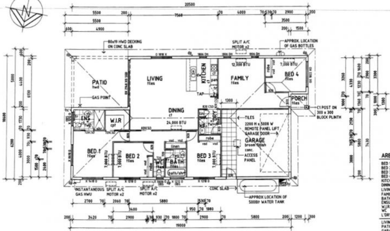
1 FLOOR PLAN 1:100
